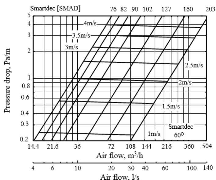
Pressure drop at 60°
