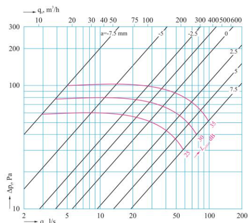
DVSC-P 160 mm
