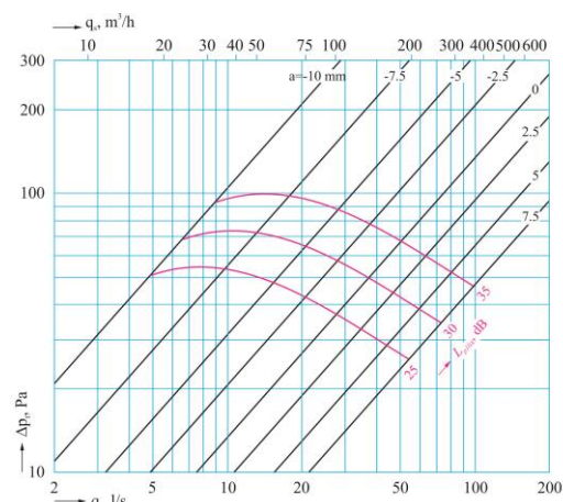
DVSC-P 150 mm
