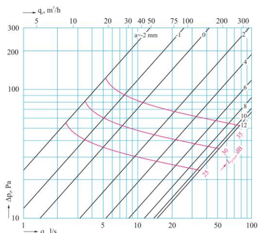
DVSC-P 100 mm
