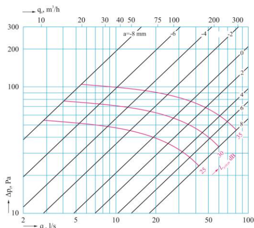
DVSC-P 125 mm
