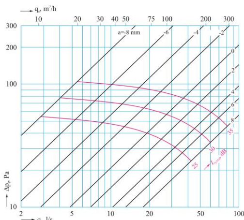
DVS-PY 125 mm
