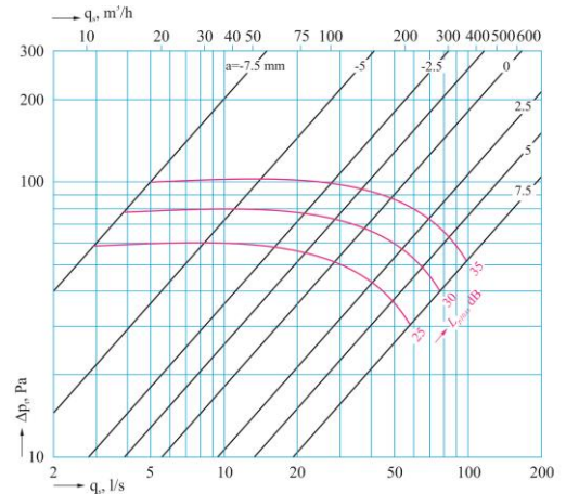
DVS-PY 160 mm
